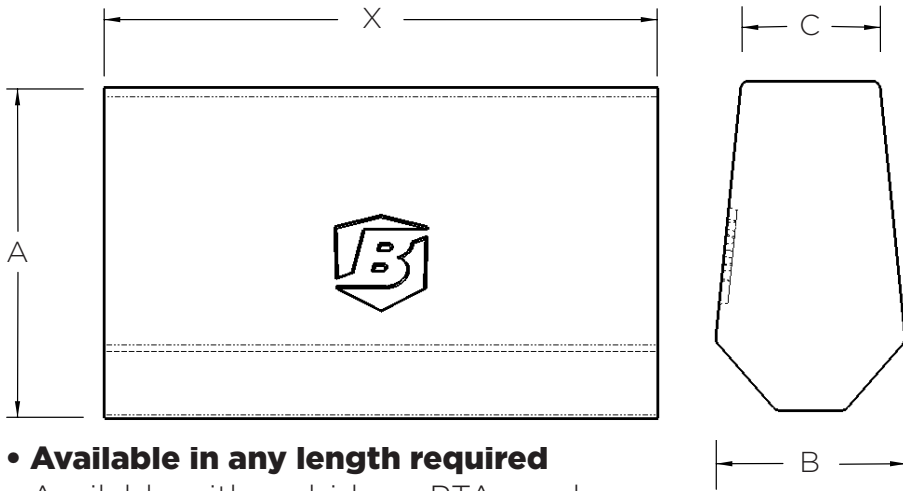
Carbide Overlay
